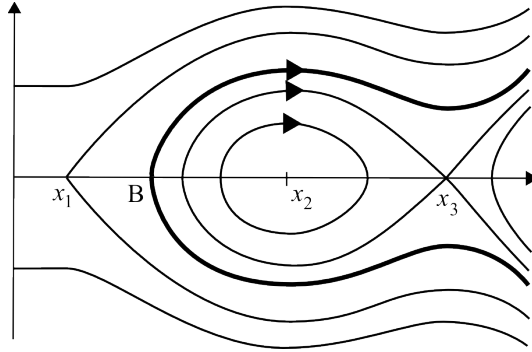
Figure 1: The escape orbit.
